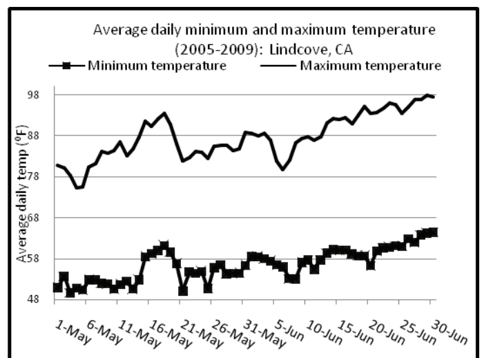
Fig 1. Average minimum and maximum temperatures recorded in Lindcove, CA from 2005-2009. Data was collected from California Irrigation Management Information System (CIMIS):
