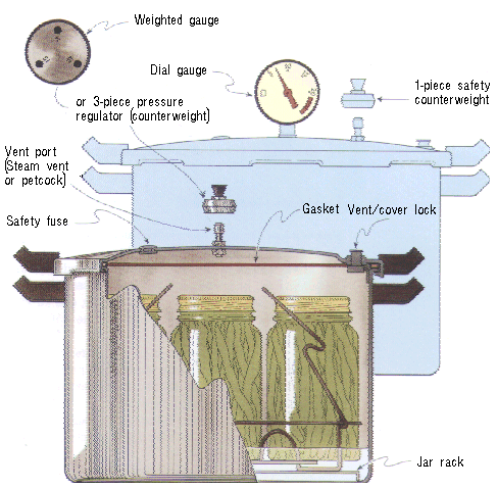
Pressure Canner
